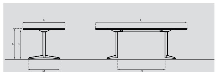
Stars oval
